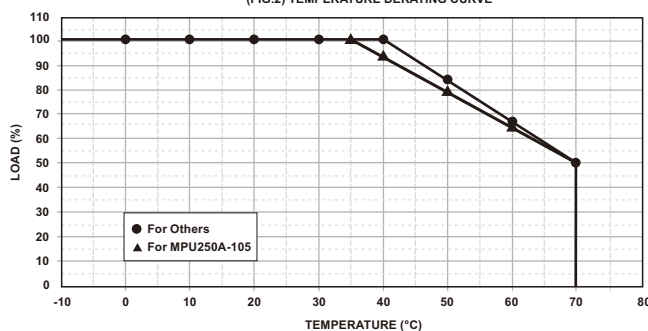
(FIG.3) TEMPERATURE DERATING CURVE
